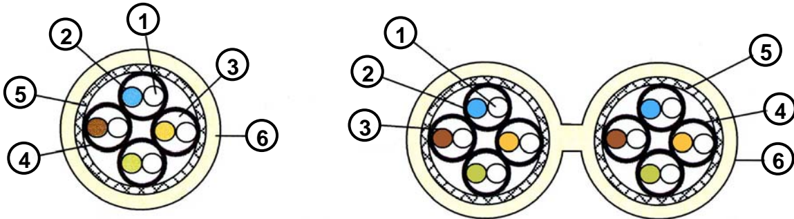
Cable construction
